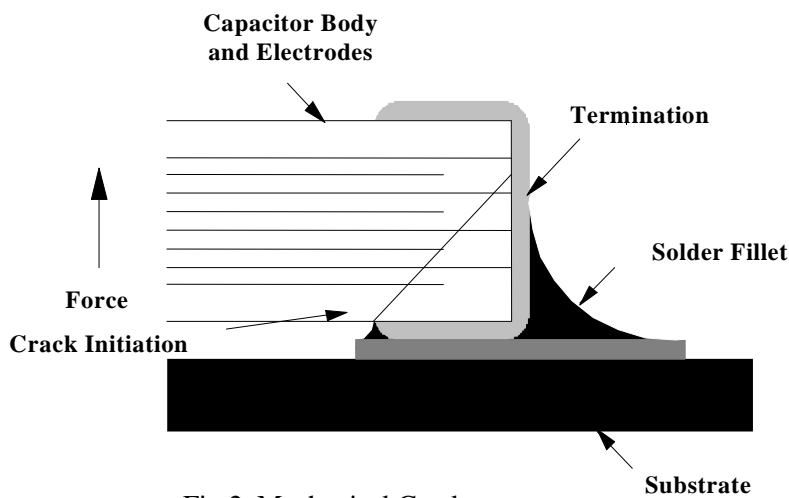
Fig 2. Mechanical Crack
