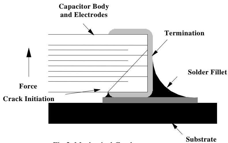
Fig 2. Mechanical Crack
