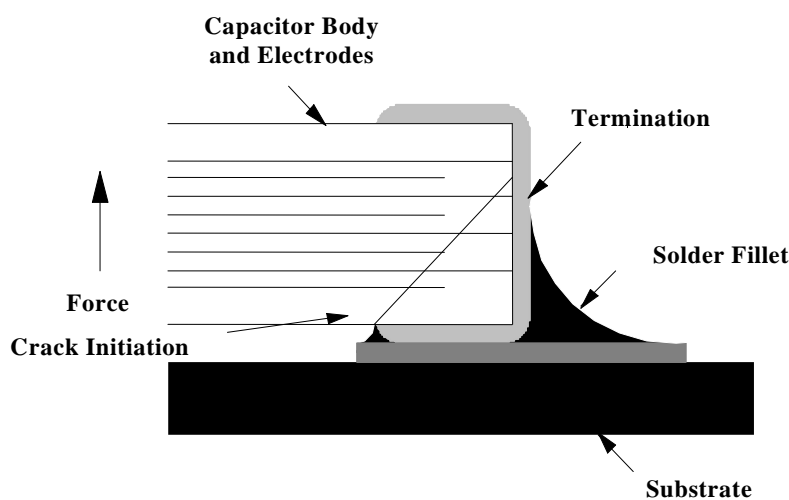
Fig 1. Mechanical Crack
